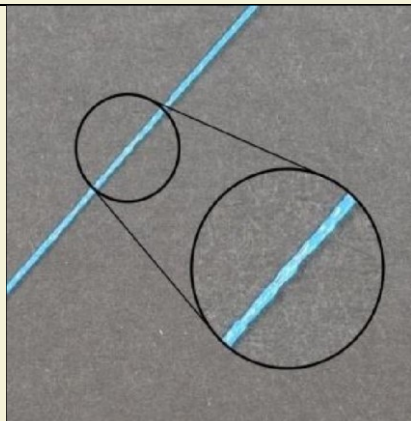
Inconsistent Extrusion
